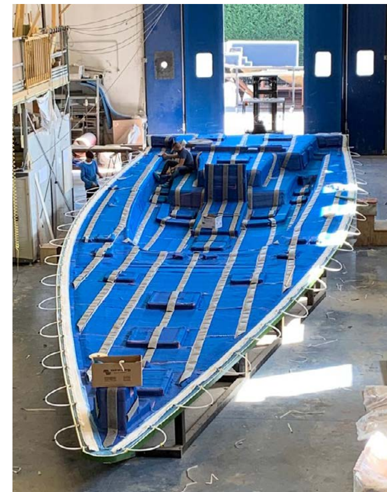
IceYachts 52RS FULL CARBON BLANKET INFUSION PREPARATION
